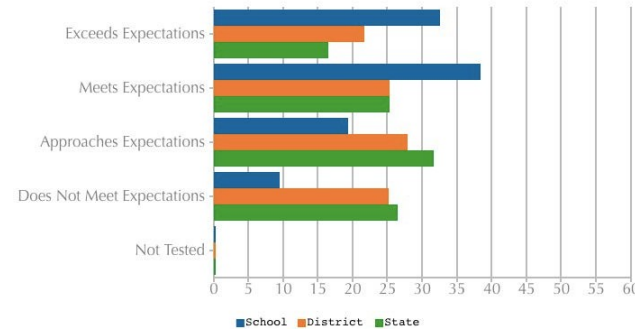
Mathematics
